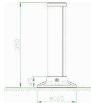
Fig 1. Install on the shoulder and fixed with the expansion screw
