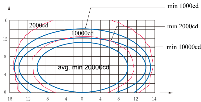
EUL-AP(White), ICAO Figure A2-1 (Vertical main beam coverage 0°—11°)
